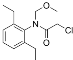
alaclor
