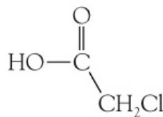
chloroacetic acid
