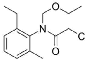
acetoclor
