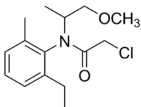
metolaclor
