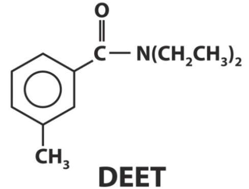
N,N-diethyl-3-metiltoluammide
